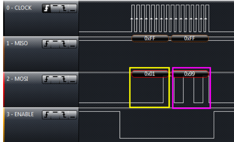
Figure 4-8. Waveform Graph 4
