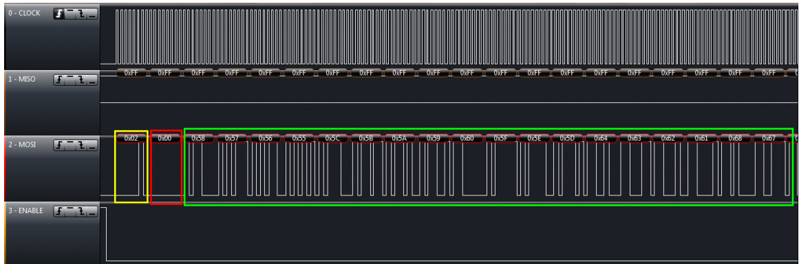
Figure 4-5. Waveform Graph 1
