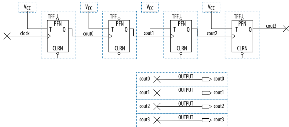
Figure 14. 4-Bit Counter Example
