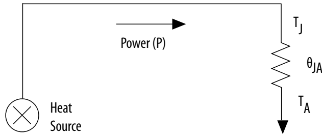
Figure 7. Thermal Model in the PowerPlay EPE Spreadsheet without a Heat Sink
