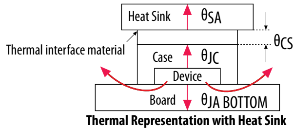
Figure 9. Thermal Representation with a Heat Sink
