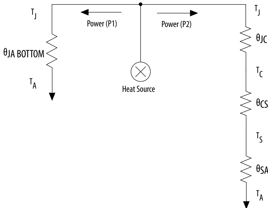
Figure 10. Thermal Model for the PowerPlay EPE Spreadsheet with a Heat Sink
