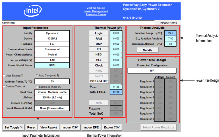
Figure 1. Main Worksheet of the PowerPlay EPE Spreadsheet
