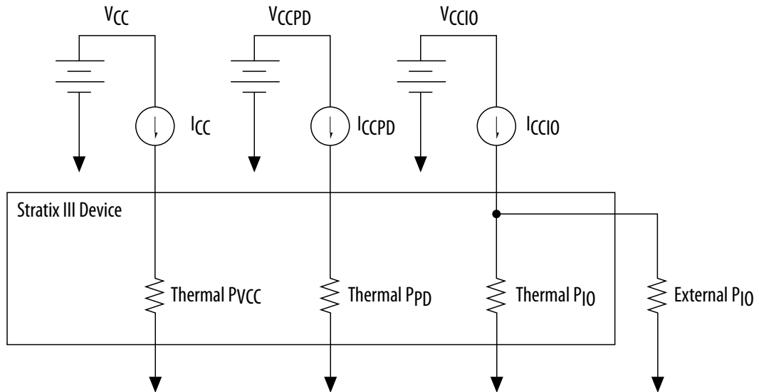
Figure 19. I/O Power Representation
