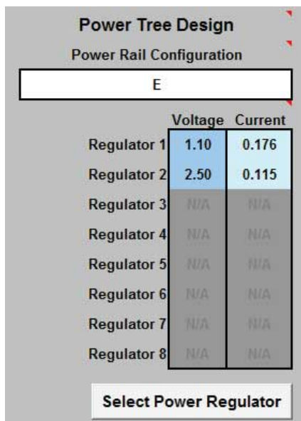
Figure 3. Power Tree Design Section in the Main Worksheet
