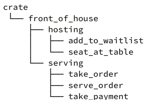
Listing 7-2: The module tree for the code in Listing 7-1
