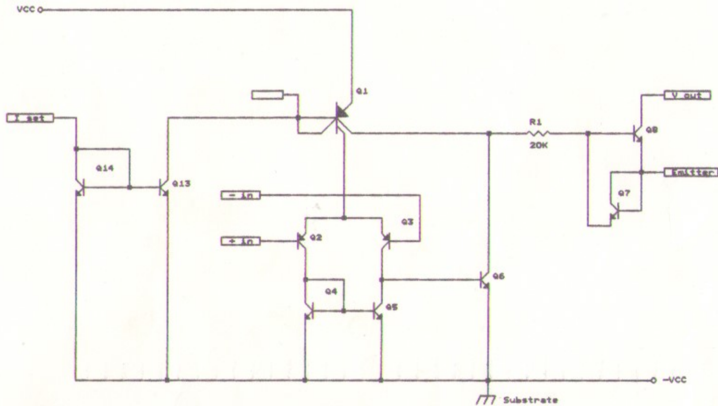
MCM4 SCHEMATIC DIAGRAM
