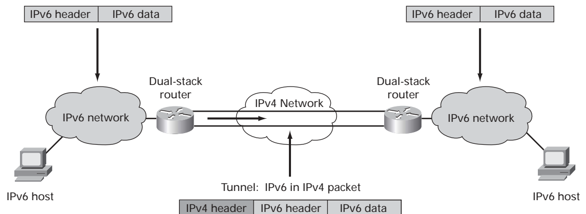
Figure 19: IPv4-IPv6 Dual Stack Operation
