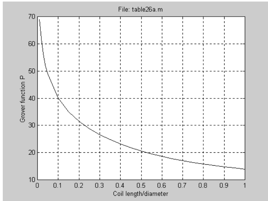
(c) Function P, for disk coils Figure 5. Circular coil with rectangular cross section
