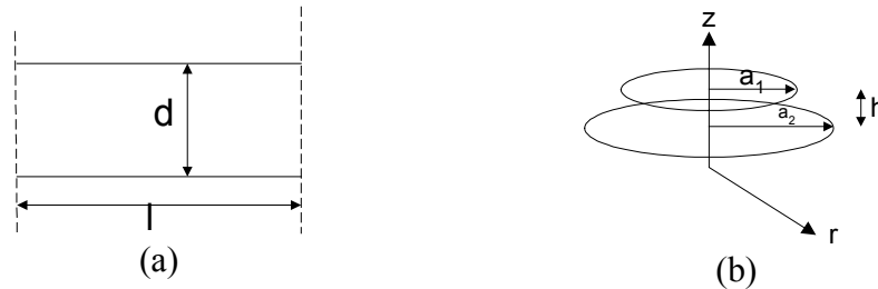
Figure 4. Mutual inductance between filaments. (a) Straight conductors (b) Loops For the coaxial loops, the mutual inductance between loops as found by Maxwell is:
