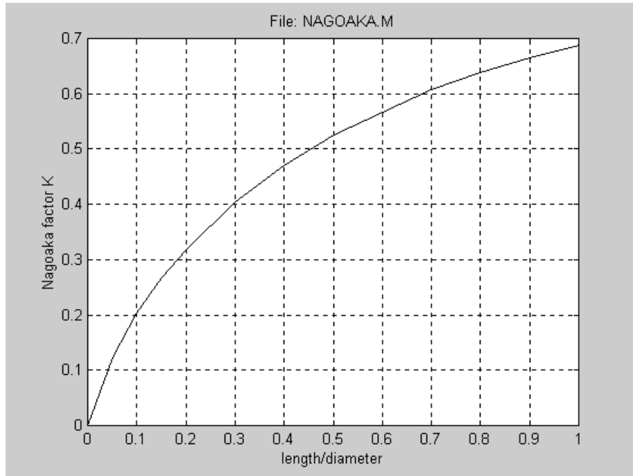
Figure 6. Correction factor for finite-length solenoid
