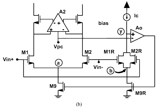
Fig. 4. (a) Basic concept of replica-tail feedback. (b) Circuit realization of replica-tail feedback.
