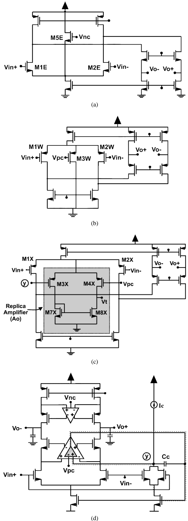
Fig. 5. Gain amp across p -channel cascodes. (b) and (c) Gain amp across n -channel cascodes. (d) Overall implementation.
