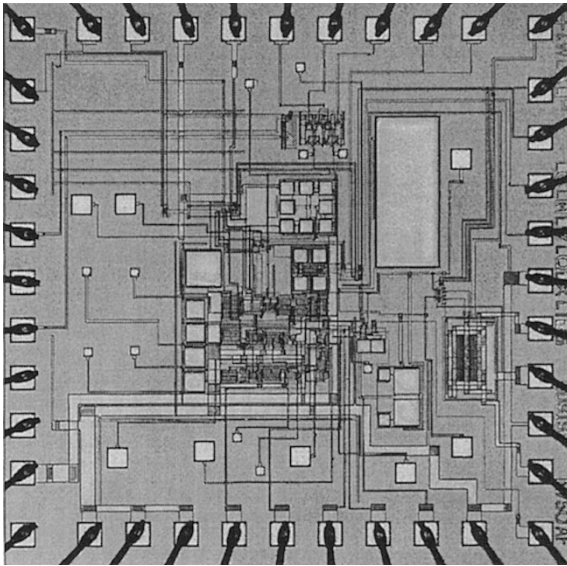
Fig. 8. Op-amp microphotograph.
