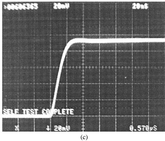
Fig. 10. Step response of op-amp. (a) Test setup. (b) Small-signal step response. (c) Large-signal step response (horizontal: 20 ns/div; vertical: 200 mV/div considering picoprobe attenuation).
