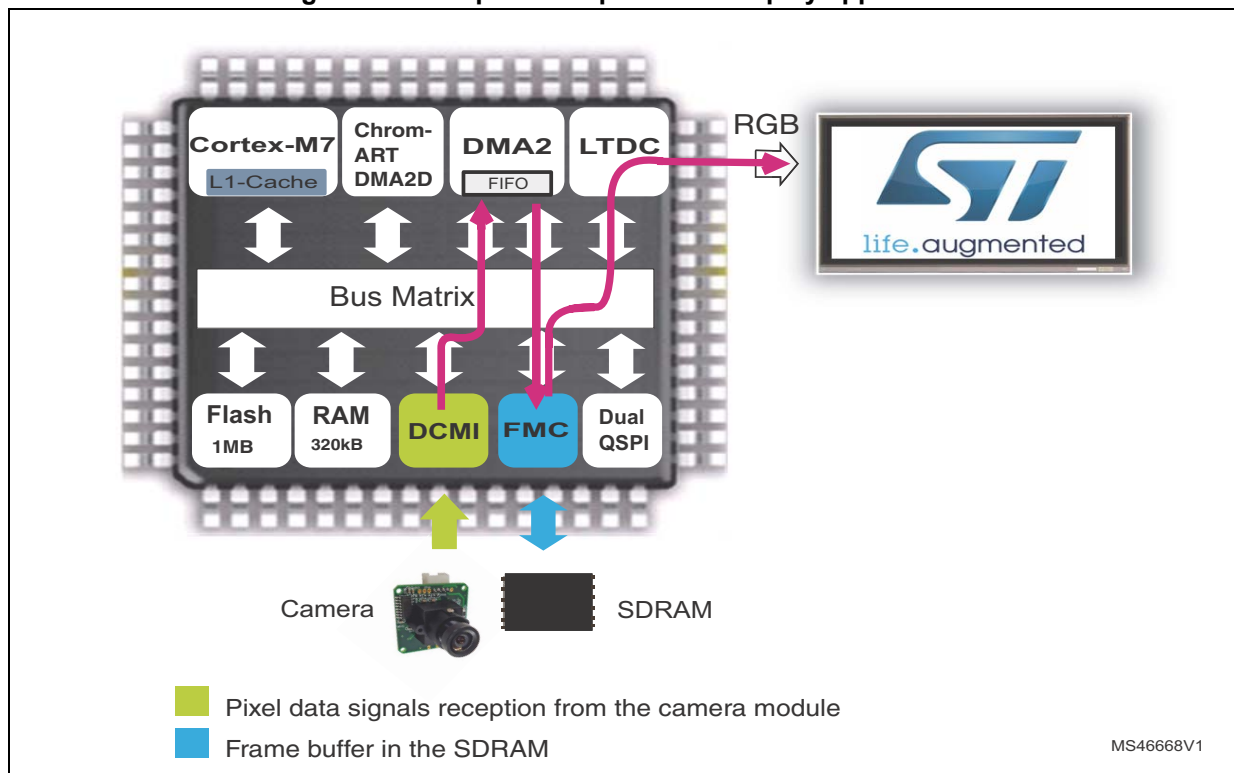
Figure 44. Data path in capture and display application
