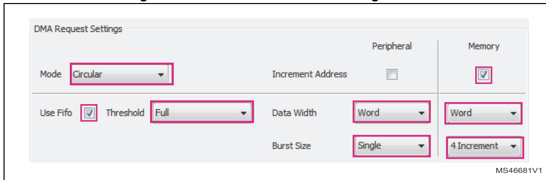
Figure 60. STM32CubeMX - DMA configuration
