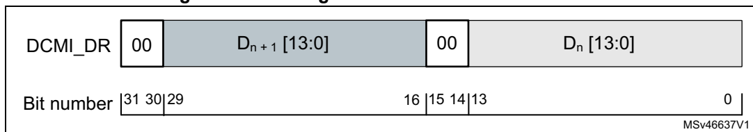
Figure 16. Data register filled for 14-bit data width
