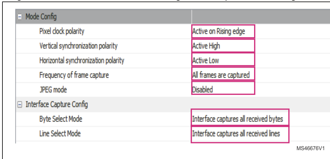
Figure 55. STM32CubeMX - DCMI control signals and capture mode configuration
