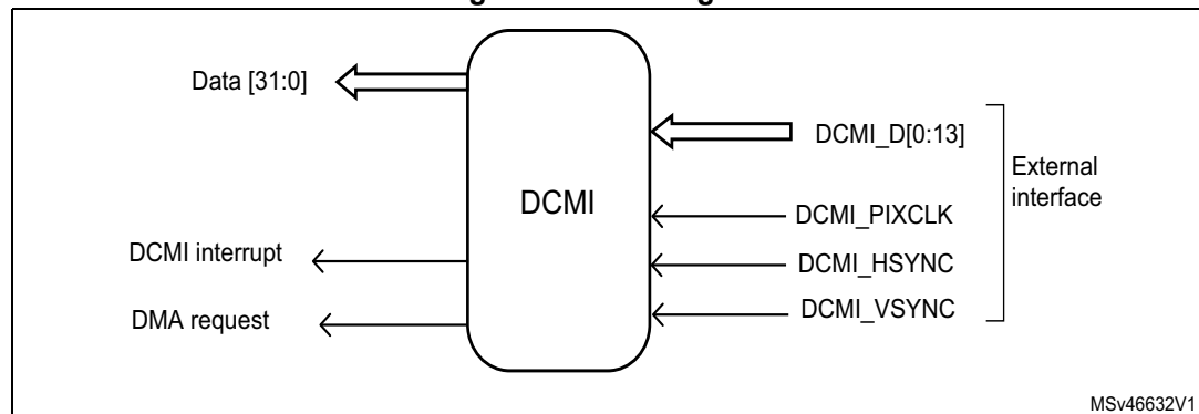
Figure 11. DCMI signals
