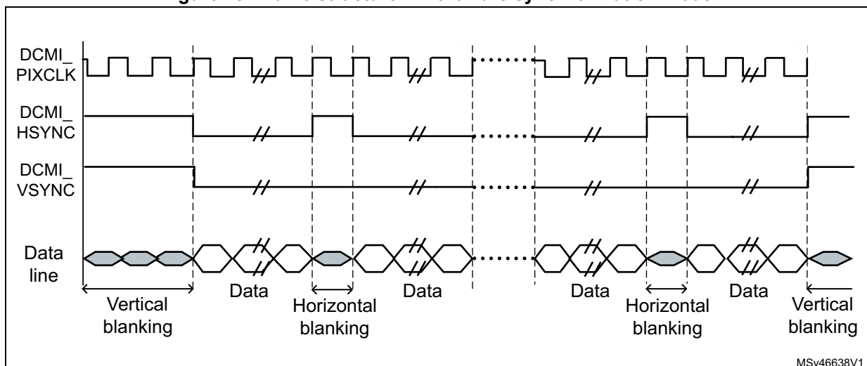
Figure 18. Frame structure in hardware synchronization mode
